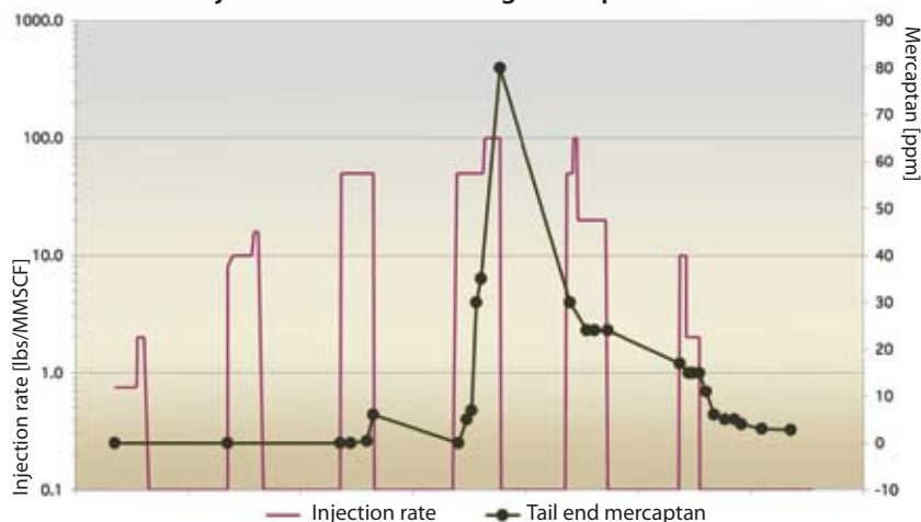
Odorant Injection Rate & Resulting Mercaptan Concentrations
